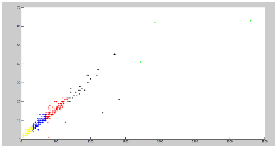
Fig3. Cluster plot about the customer dataset based on FCM
