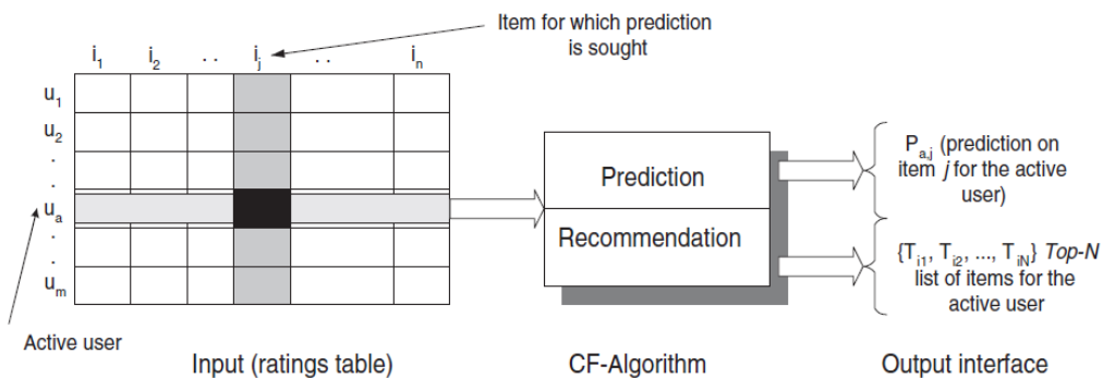
Fig2. The Collaborative Filtering Process (sourced from literature [8])
